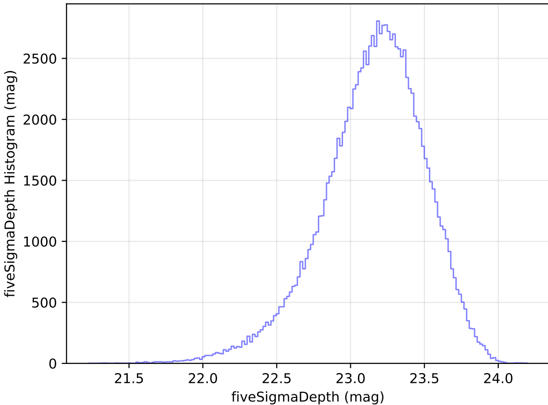
roman_v3.3_10yrs u: fiveSigmaDepth Histogram
