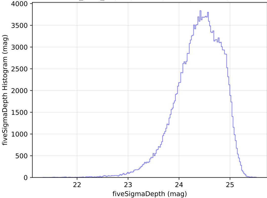
roman_v3.3_10yrs g: fiveSigmaDepth Histogram
