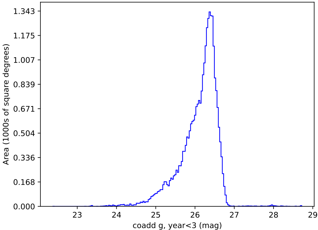
roman_v3.3_10yrs night<1095 and g: coadd g, year<3
