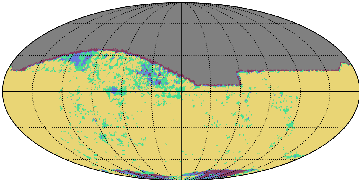
roman_v3.3_10yrs z band: YearCoverage night
