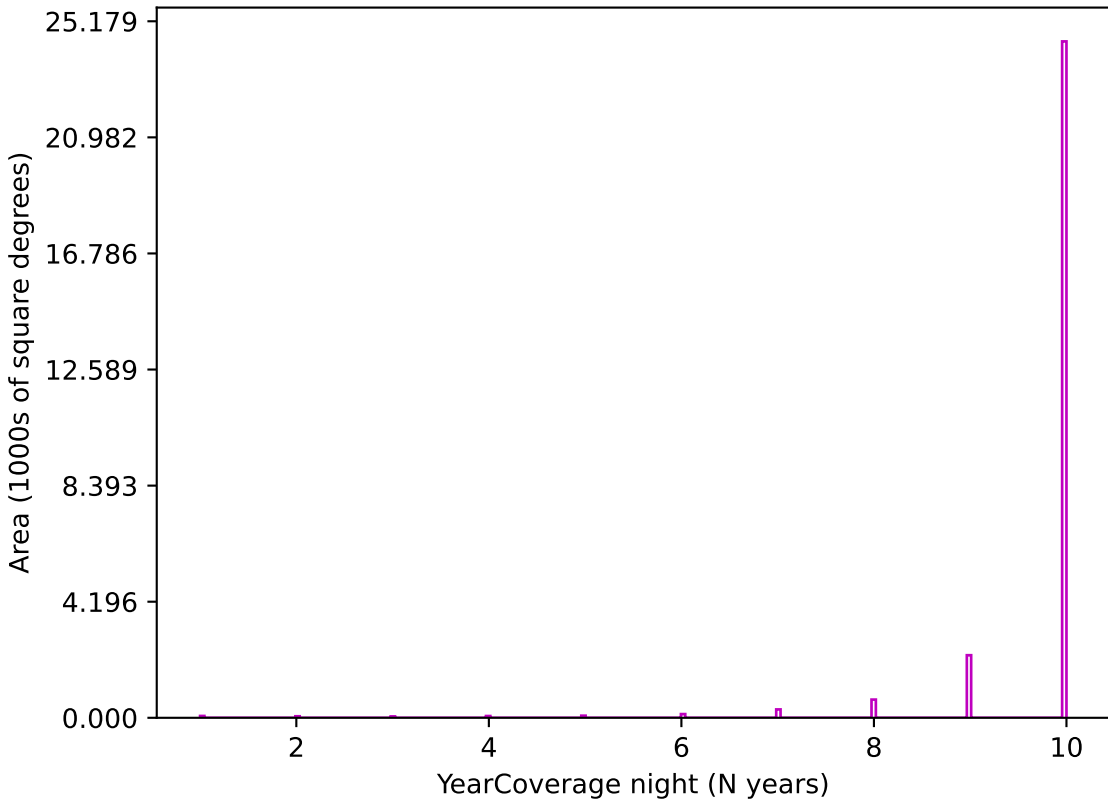
roman_v3.3_10yrs z band: YearCoverage night
