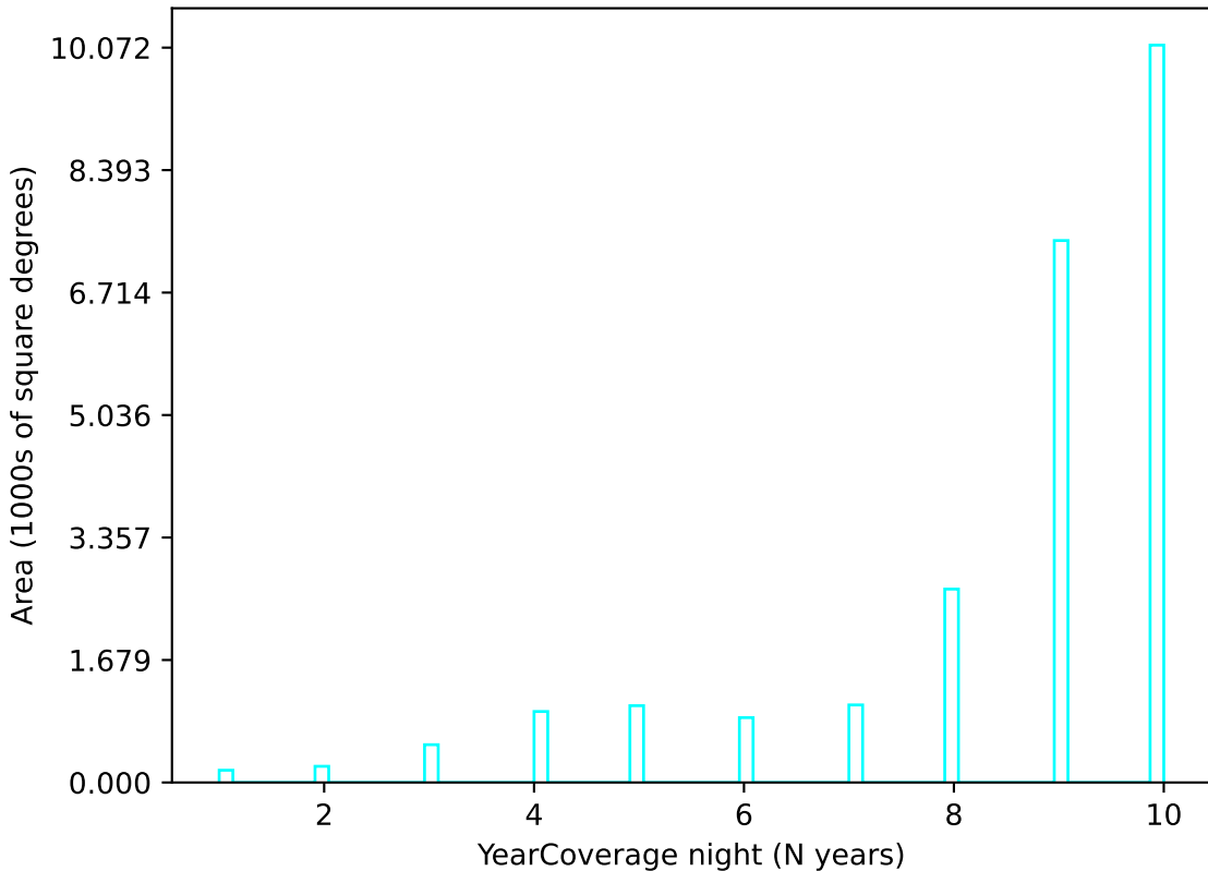
roman_v3.3_10yrs u band: YearCoverage night
