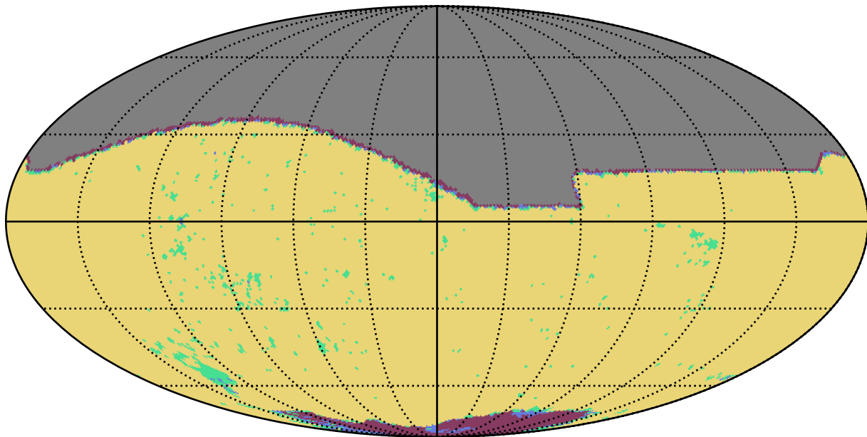
roman_v3.3_10yrs r band: YearCoverage night
