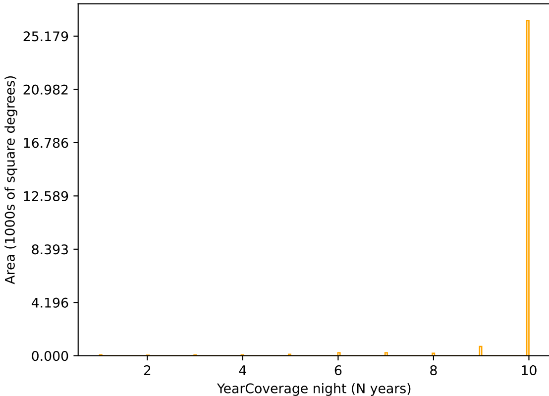
roman_v3.3_10yrs r band: YearCoverage night
