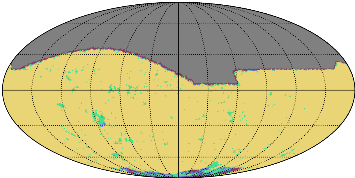
roman_v3.3_10yrs i band: YearCoverage night
