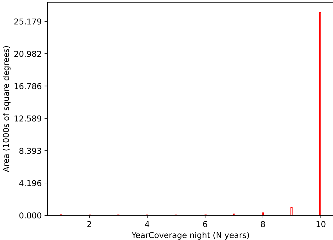
roman_v3.3_10yrs i band: YearCoverage night
