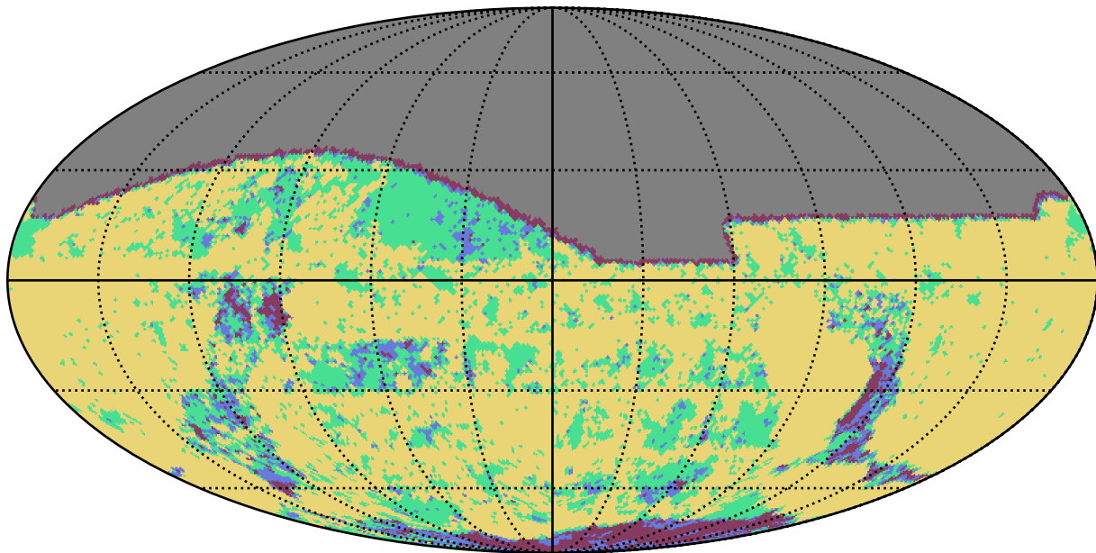
roman_v3.3_10yrs g band: YearCoverage night
