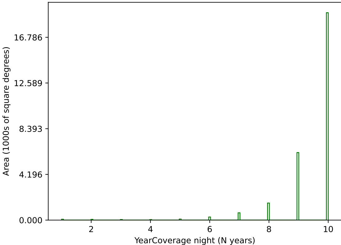
roman_v3.3_10yrs g band: YearCoverage night
