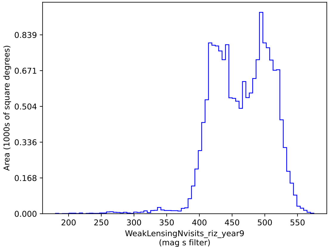
roman_v3.3_10yrs gri band non-DD: WeakLensingNvisits_riz_year9
