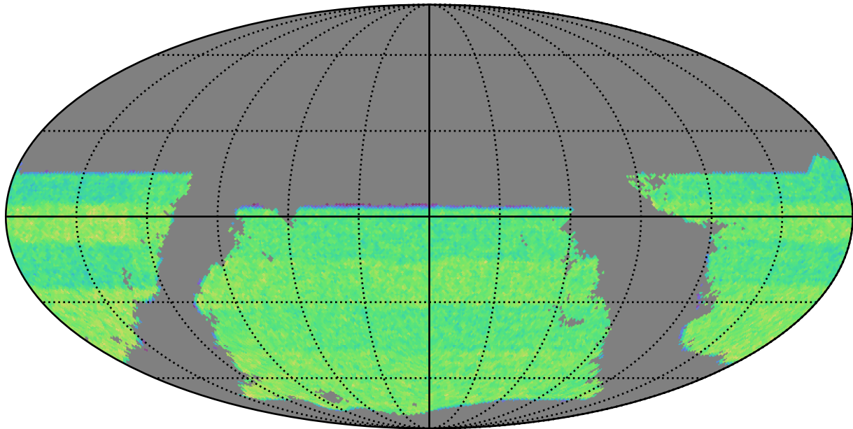
roman_v3.3_10yrs gri band non-DD: WeakLensingNvisits_riz_year8
