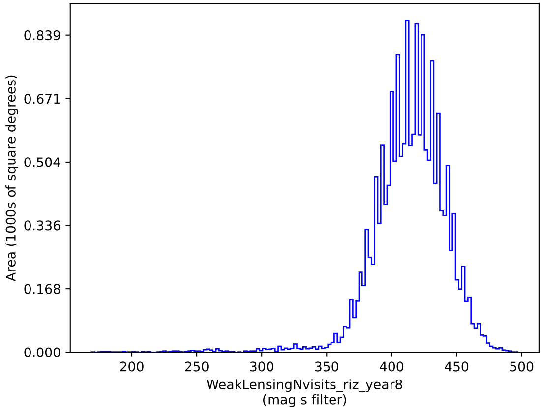
roman_v3.3_10yrs gri band non-DD: WeakLensingNvisits_riz_year8
