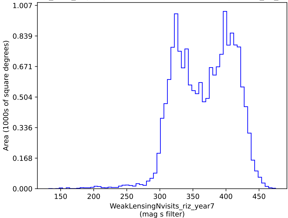
roman_v3.3_10yrs gri band non-DD: WeakLensingNvisits_riz_year7
