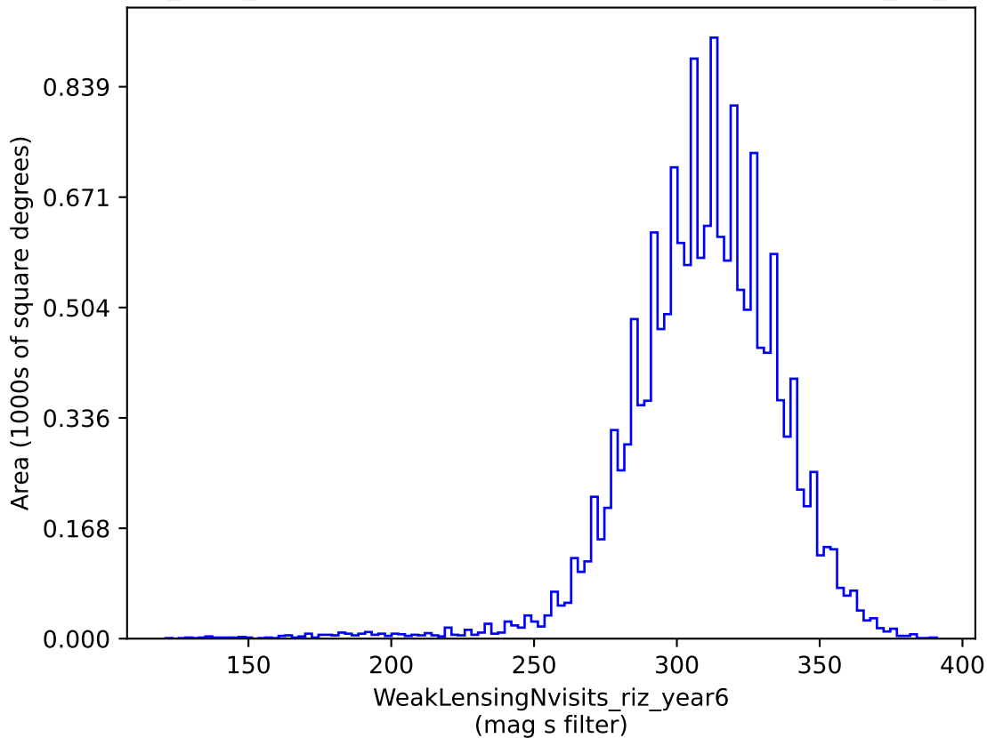
roman_v3.3_10yrs gri band non-DD: WeakLensingNvisits_riz_year6
