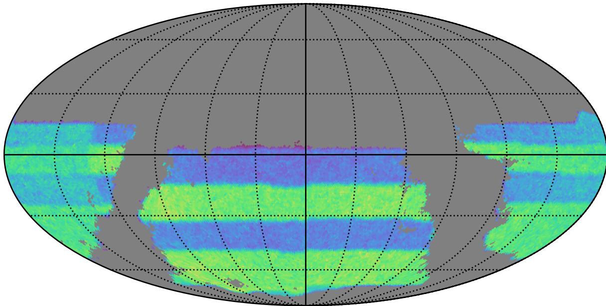
roman_v3.3_10yrs gri band non-DD: WeakLensingNvisits_riz_year3
