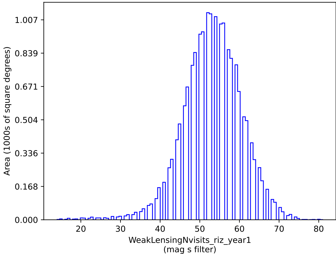
roman_v3.3_10yrs gri band non-DD: WeakLensingNvisits_riz_year1
