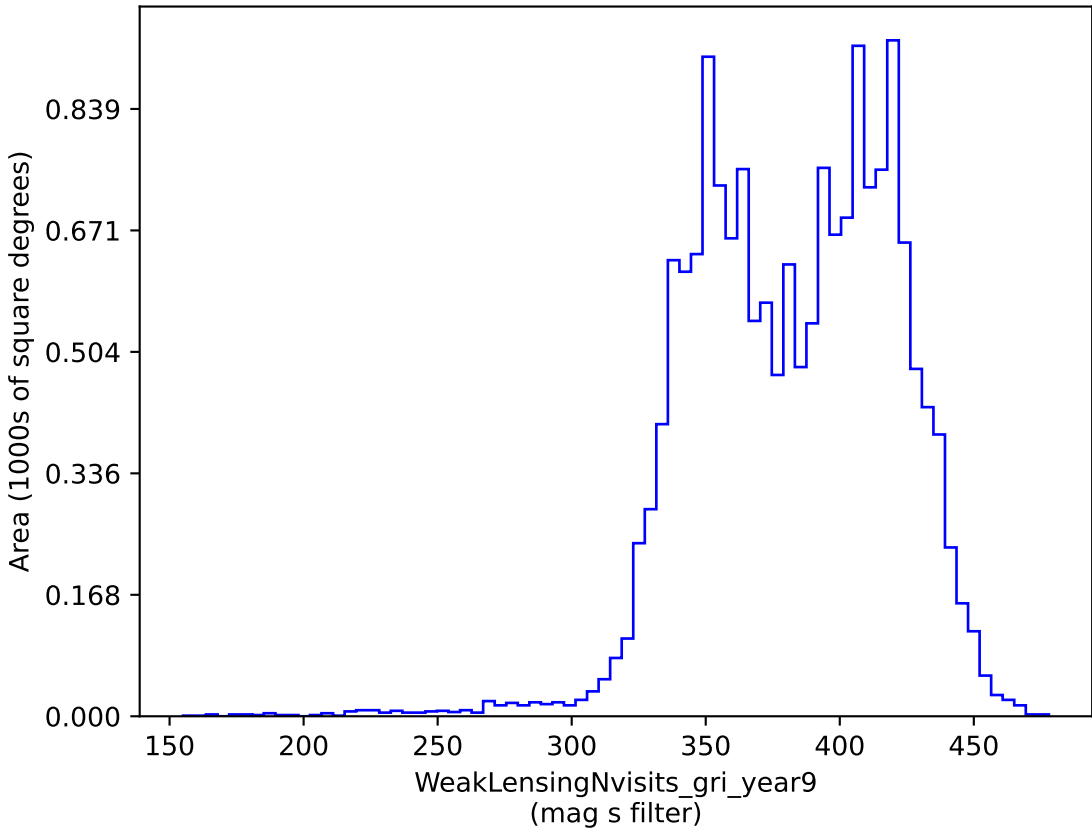
roman_v3.3_10yrs gri band non-DD: WeakLensingNvisits_gri_year9
