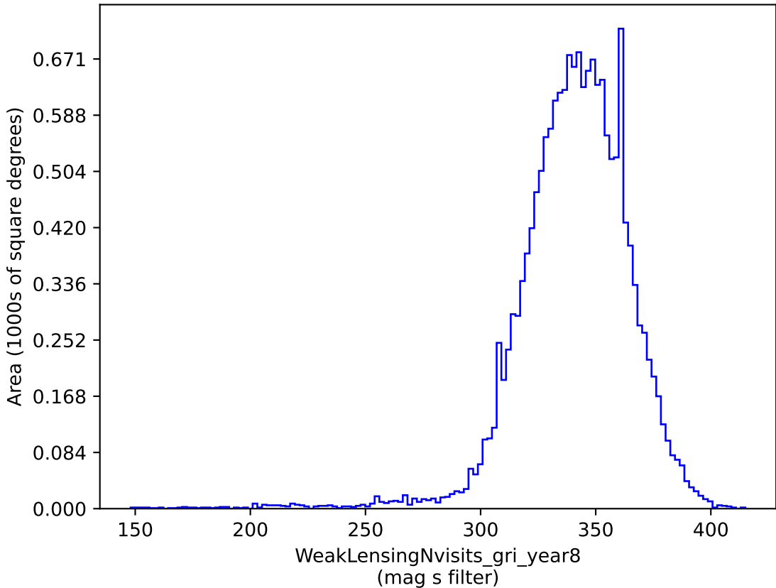
roman_v3.3_10yrs gri band non-DD: WeakLensingNvisits_gri_year8
