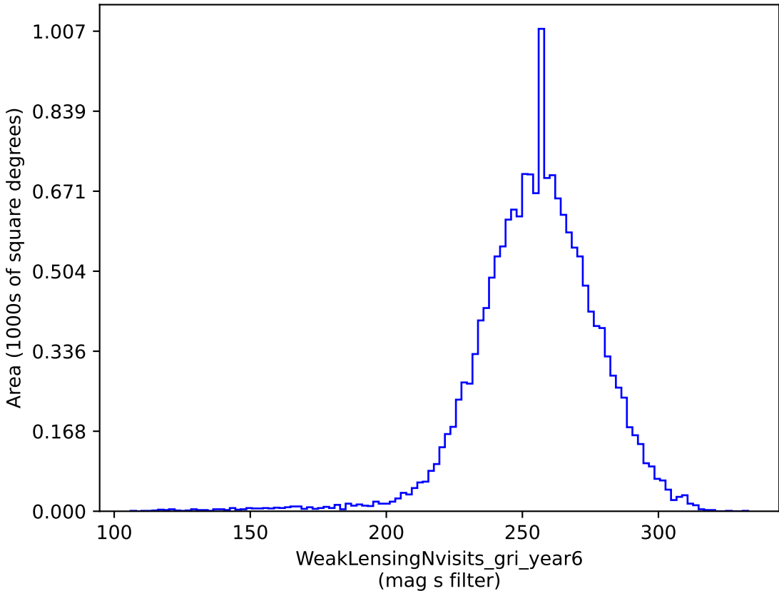
roman_v3.3_10yrs gri band non-DD: WeakLensingNvisits_gri_year6
