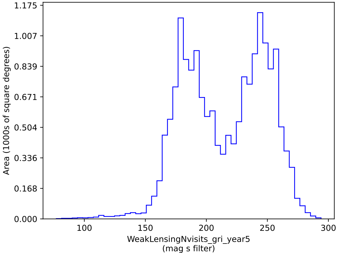
roman_v3.3_10yrs gri band non-DD: WeakLensingNvisits_gri_year5
