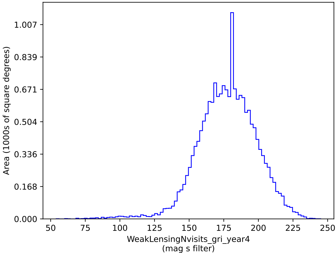
roman_v3.3_10yrs gri band non-DD: WeakLensingNvisits_gri_year4
