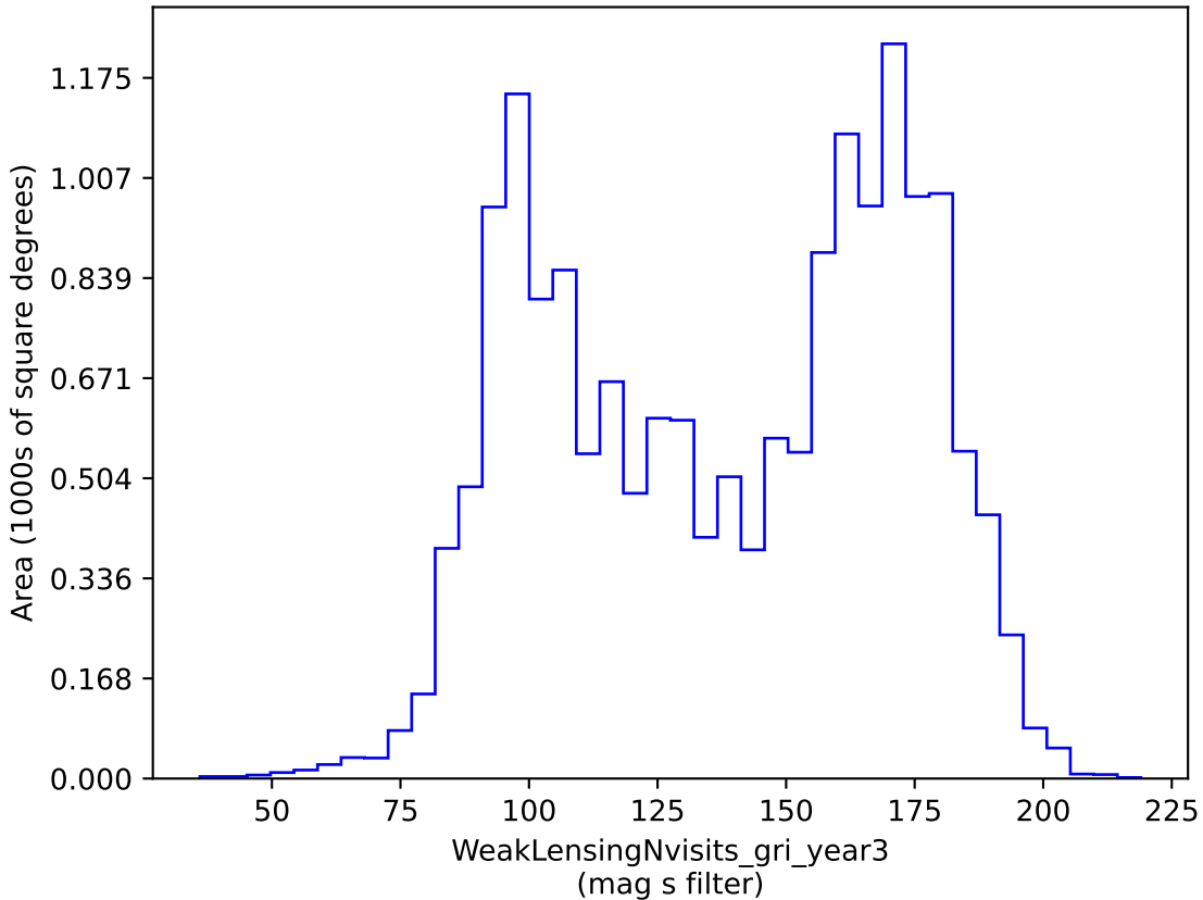
roman_v3.3_10yrs gri band non-DD: WeakLensingNvisits_gri_year3
