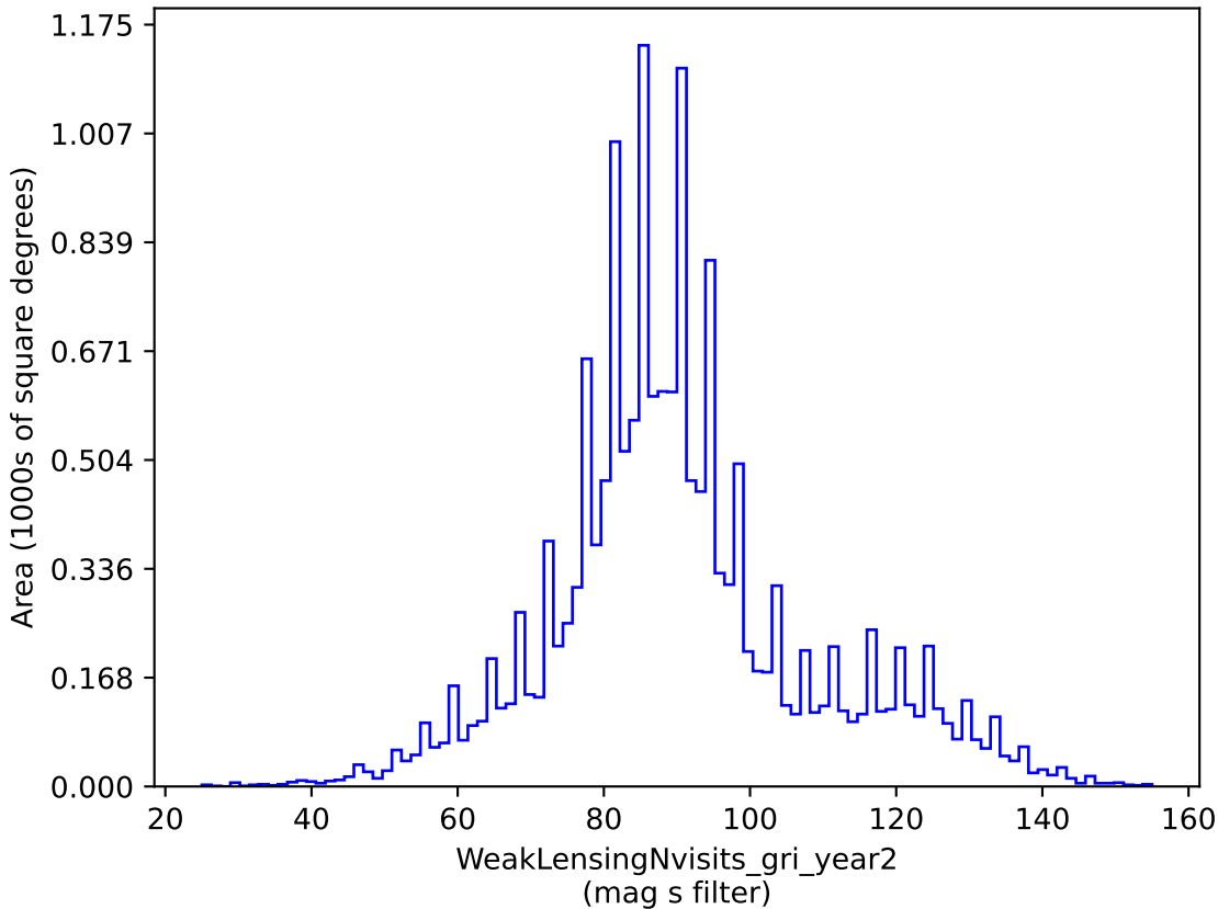
roman_v3.3_10yrs gri band non-DD: WeakLensingNvisits_gri_year2
