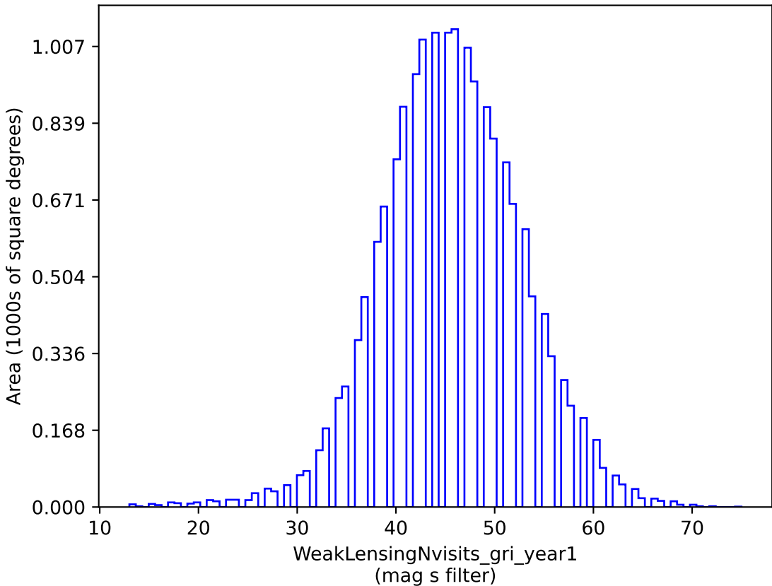
roman_v3.3_10yrs gri band non-DD: WeakLensingNvisits_gri_year1
