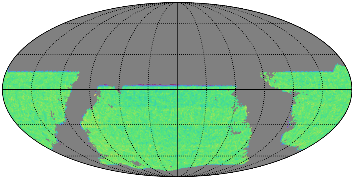
roman_v3.3_10yrs gri band non-DD: WeakLensingNvisits
