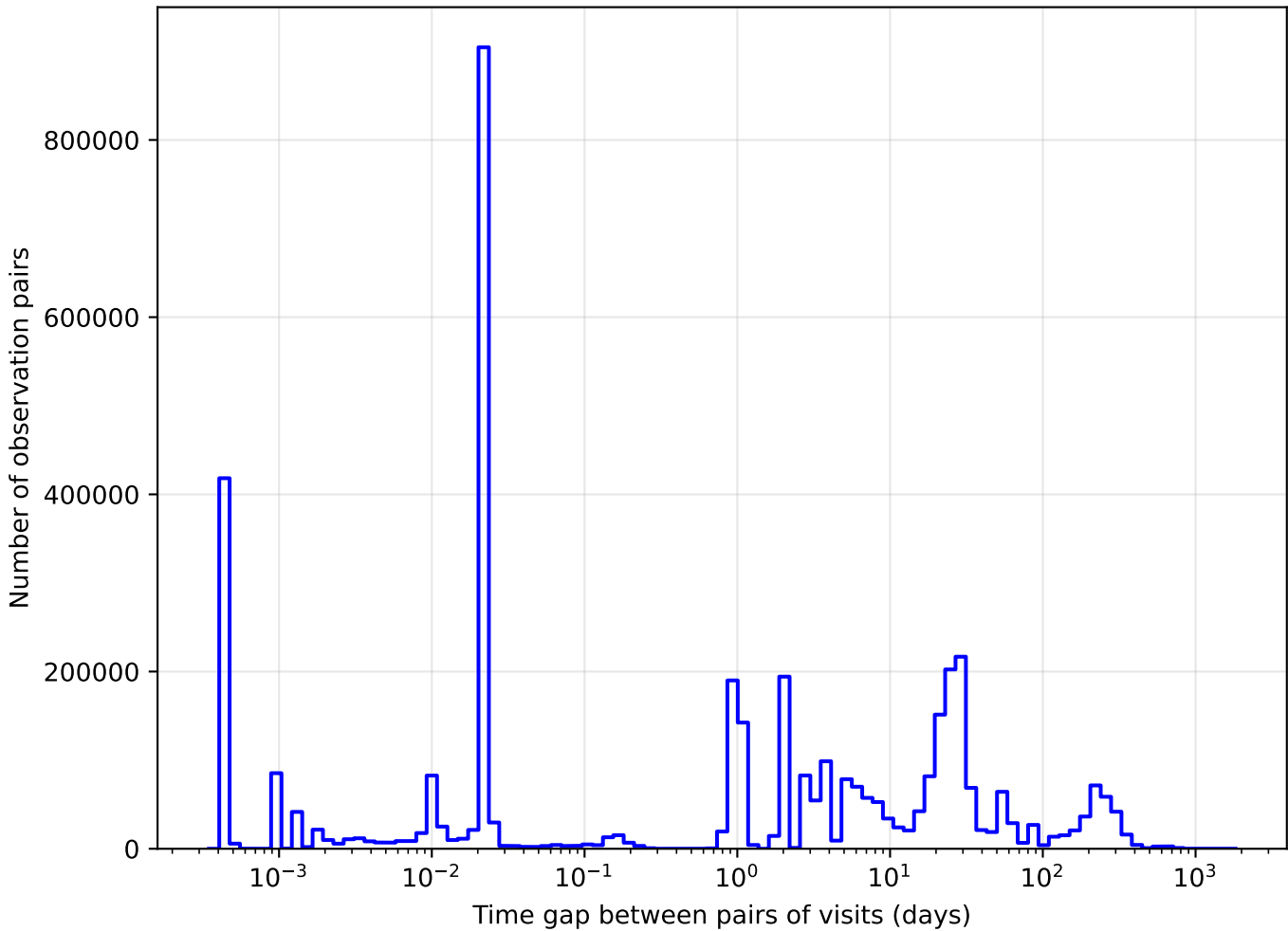
roman_v3.3_10yrs y band: Tgaps observationStartMJD
