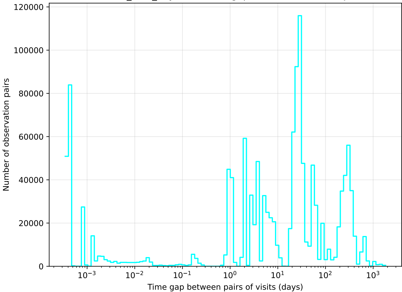
roman_v3.3_10yrs u band: Tgaps observationStartMJD
