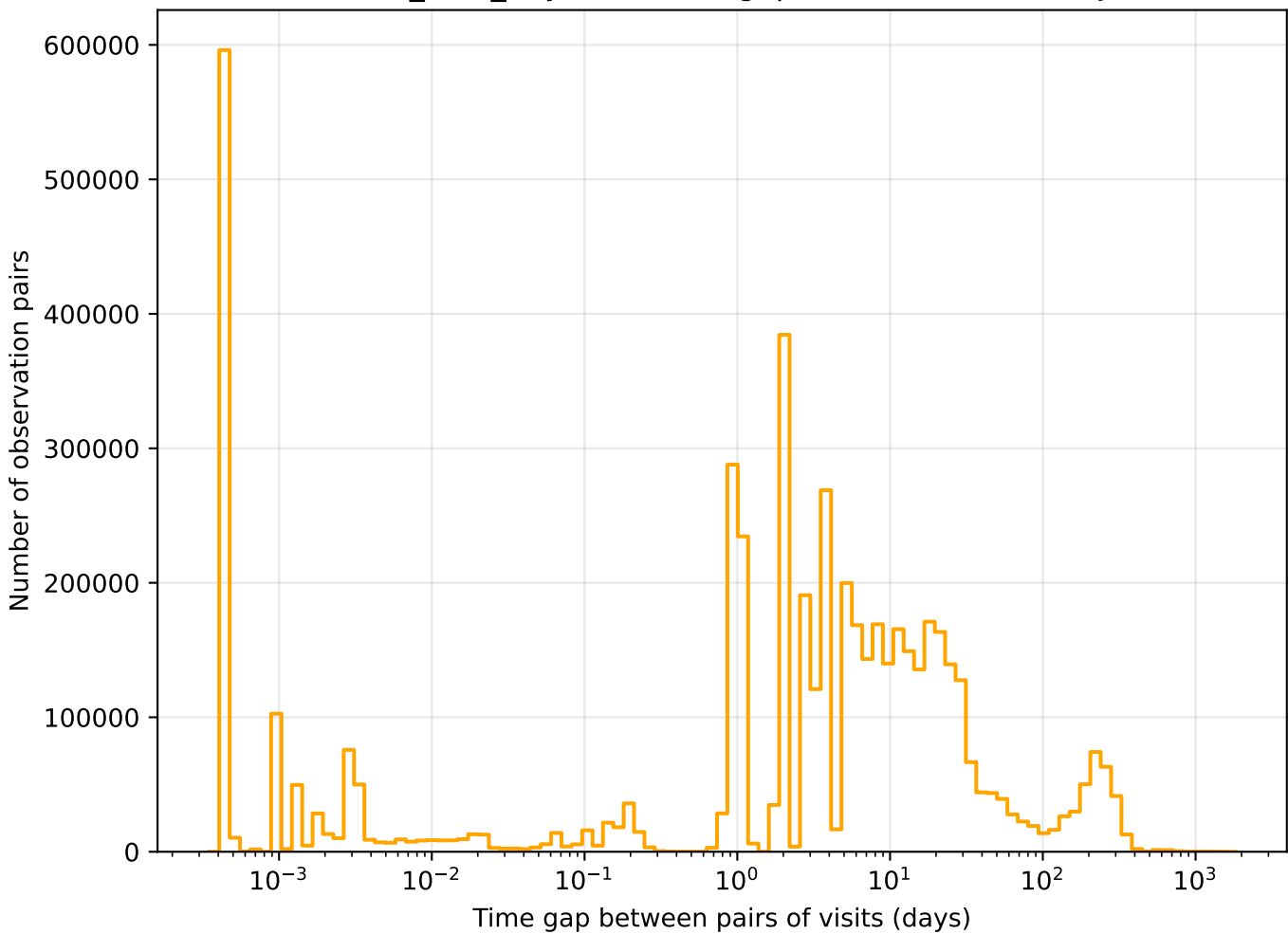
roman_v3.3_10yrs r band: Tgaps observationStartMJD
