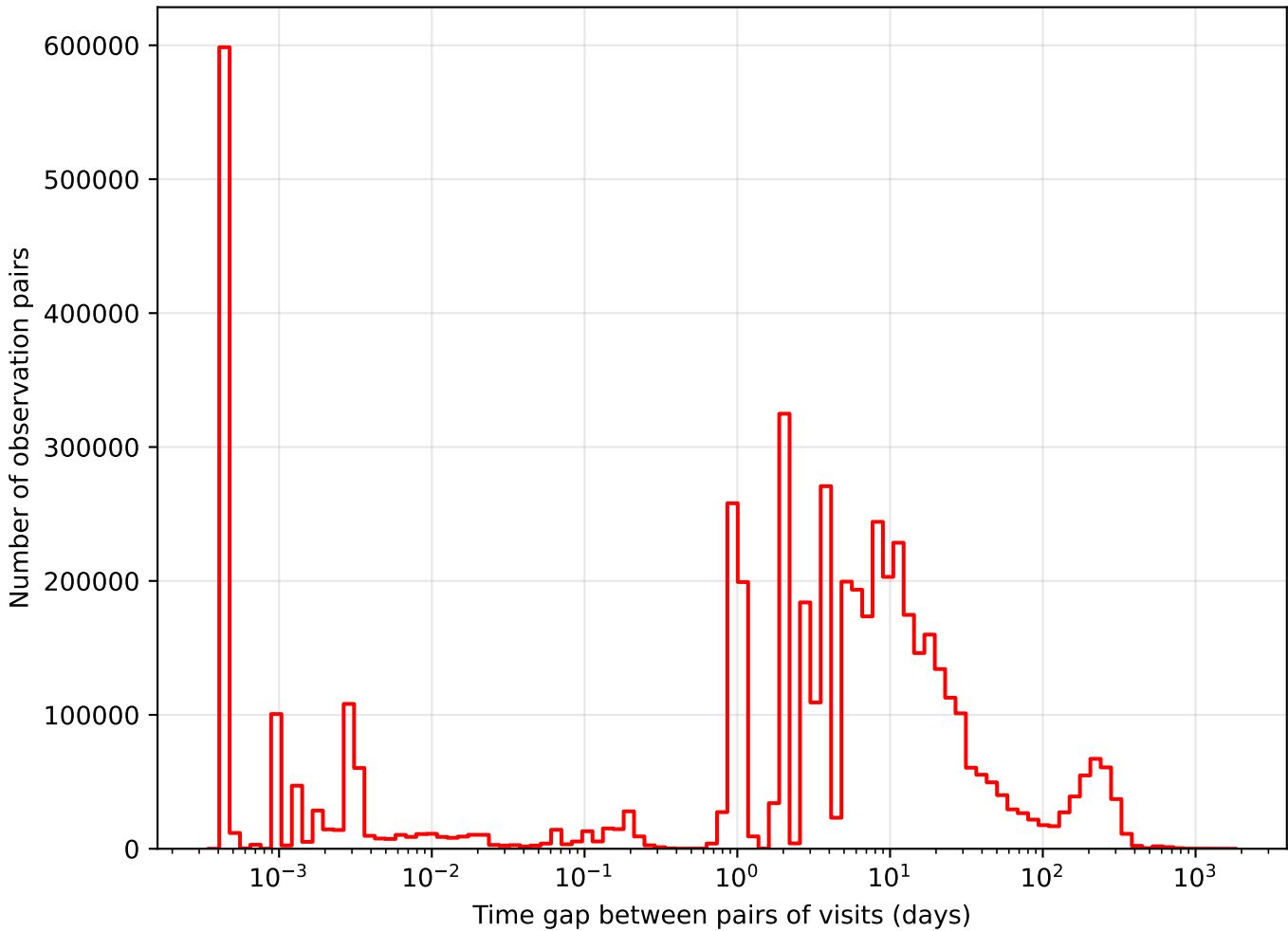
roman_v3.3_10yrs i band: Tgaps observationStartMJD
