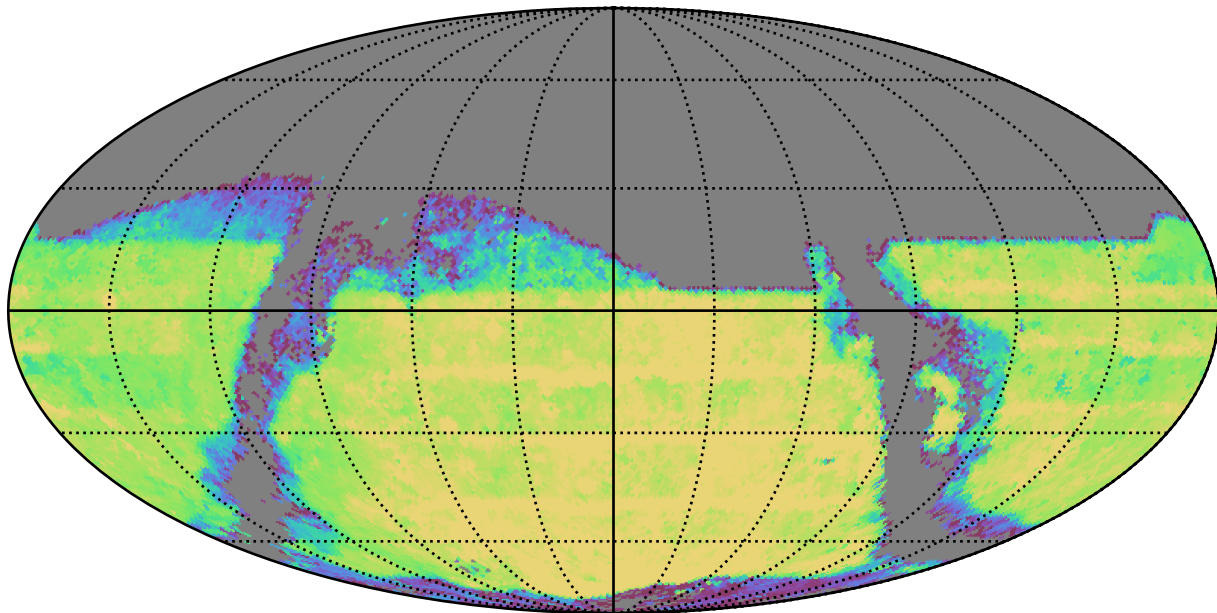
roman_v3.3_10yrs : TDC_season
