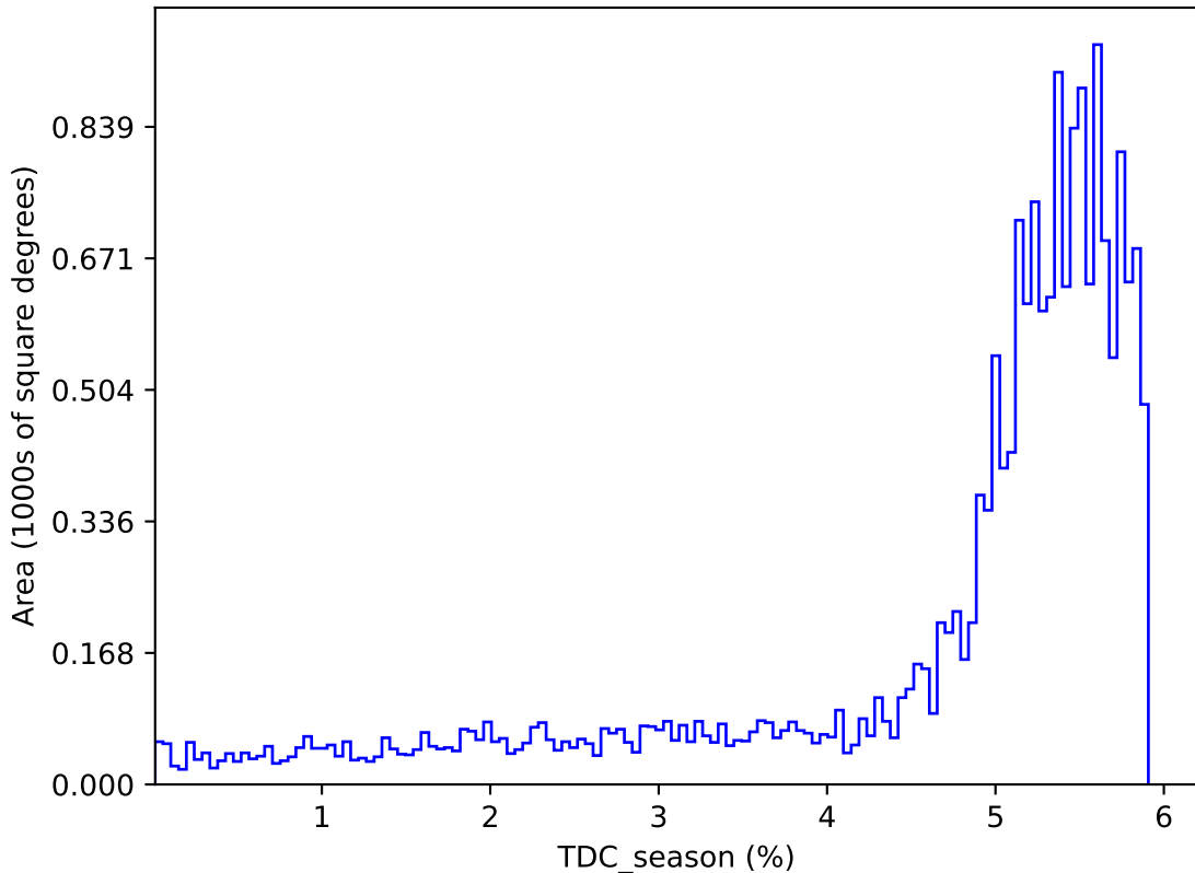
roman_v3.3_10yrs : TDC_season
