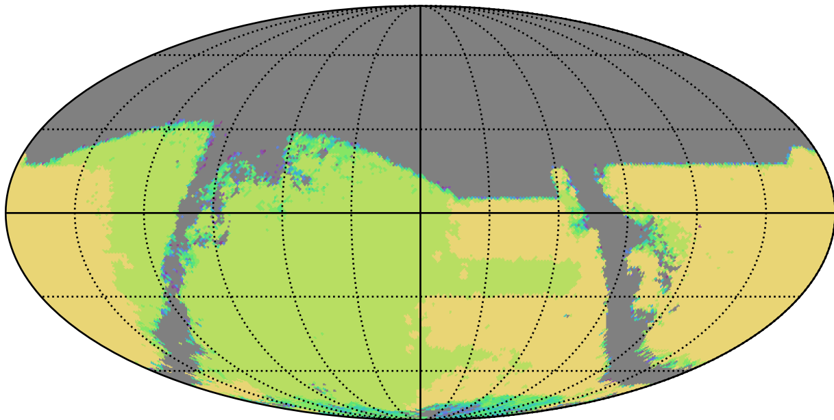
roman_v3.3_10yrs : TDC_campaign
