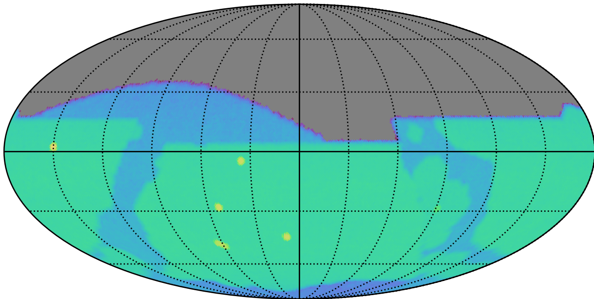
roman_v3.3_10yrs z: SurfaceBrightLimit
