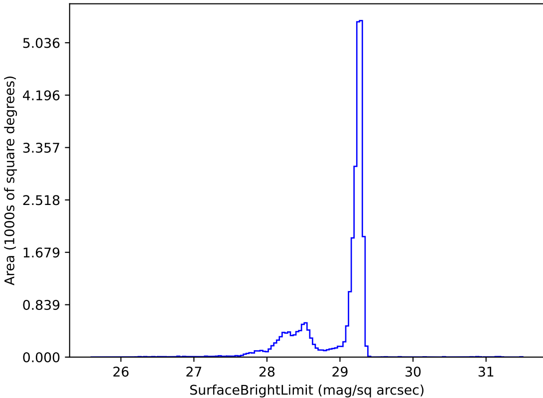
roman_v3.3_10yrs z: SurfaceBrightLimit
