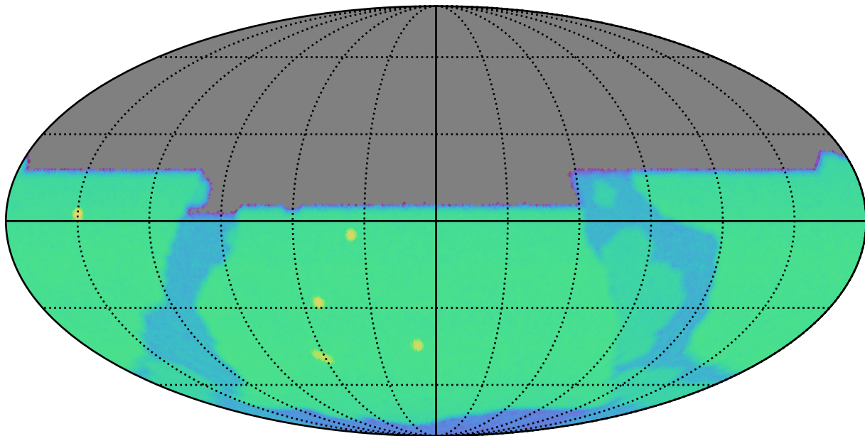
roman_v3.3_10yrs y: SurfaceBrightLimit
