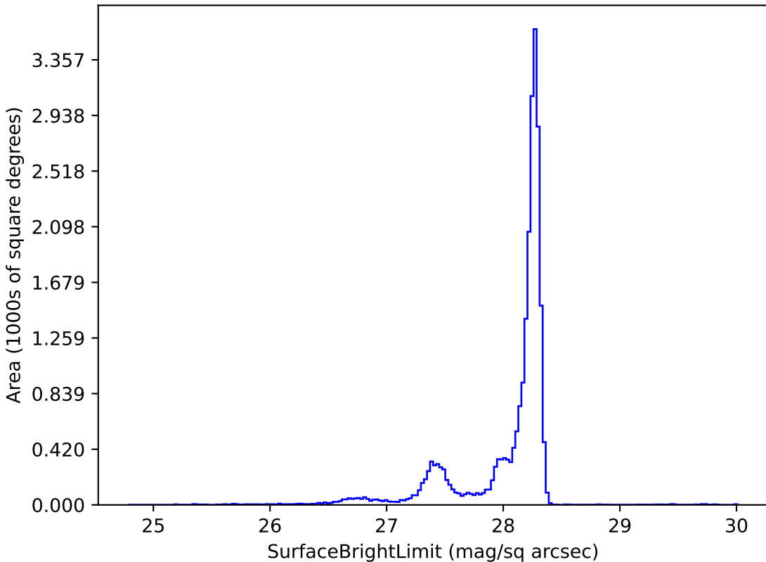
roman_v3.3_10yrs y: SurfaceBrightLimit
