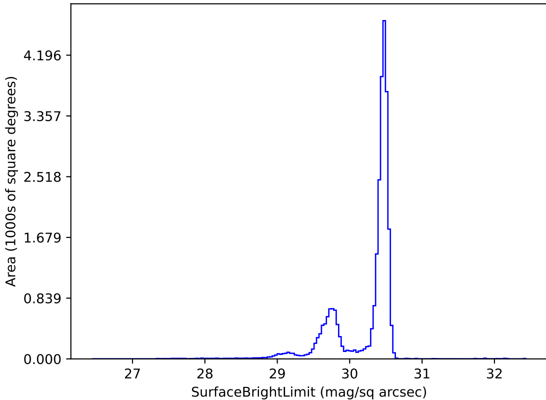
roman_v3.3_10yrs r: SurfaceBrightLimit
