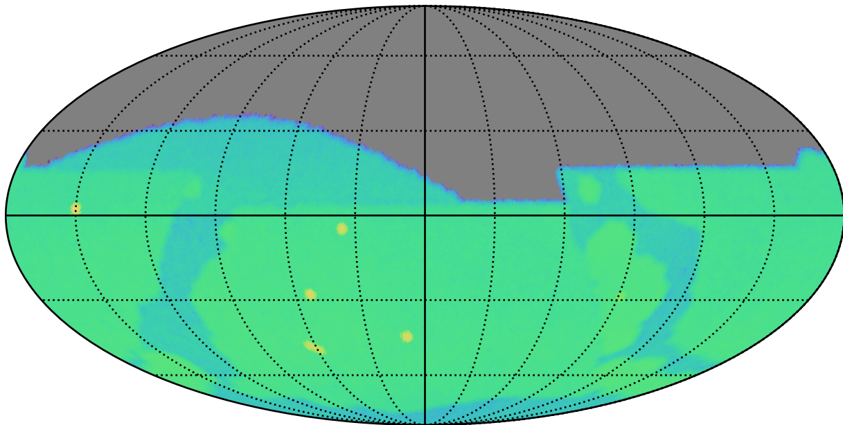
roman_v3.3_10yrs g: SurfaceBrightLimit
