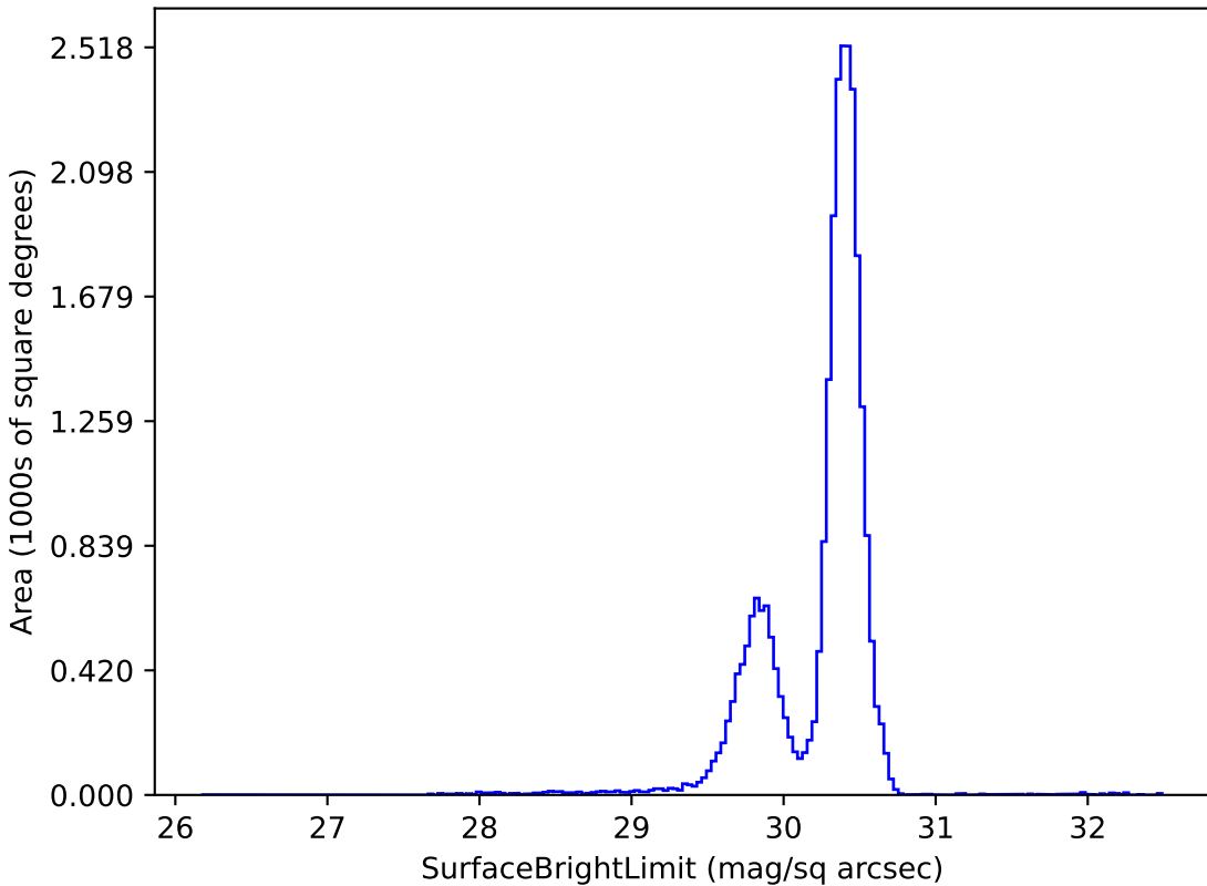
roman_v3.3_10yrs g: SurfaceBrightLimit
