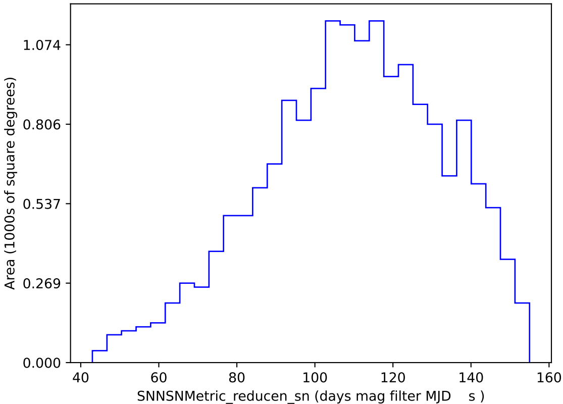
roman_v3.3_10yrs DDF excluded: SNNSNMetric_reducen_sn
