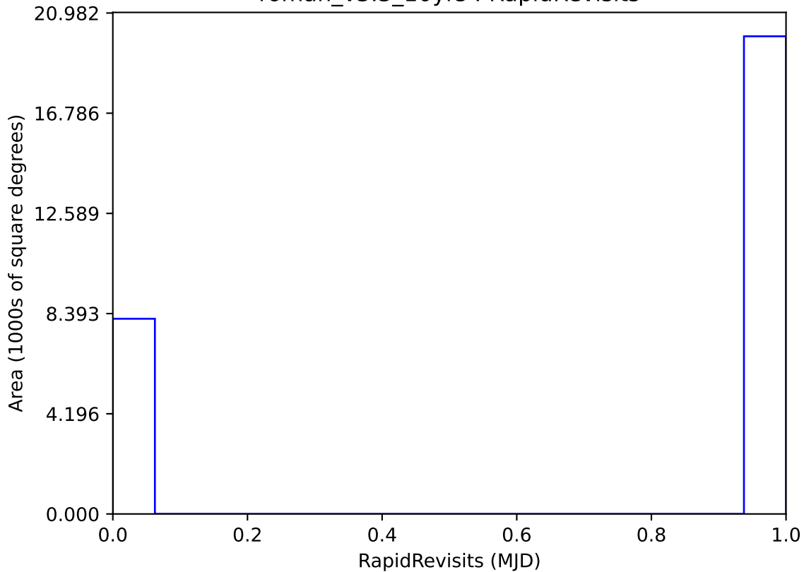
roman_v3.3_10yrs : RapidRevisits
