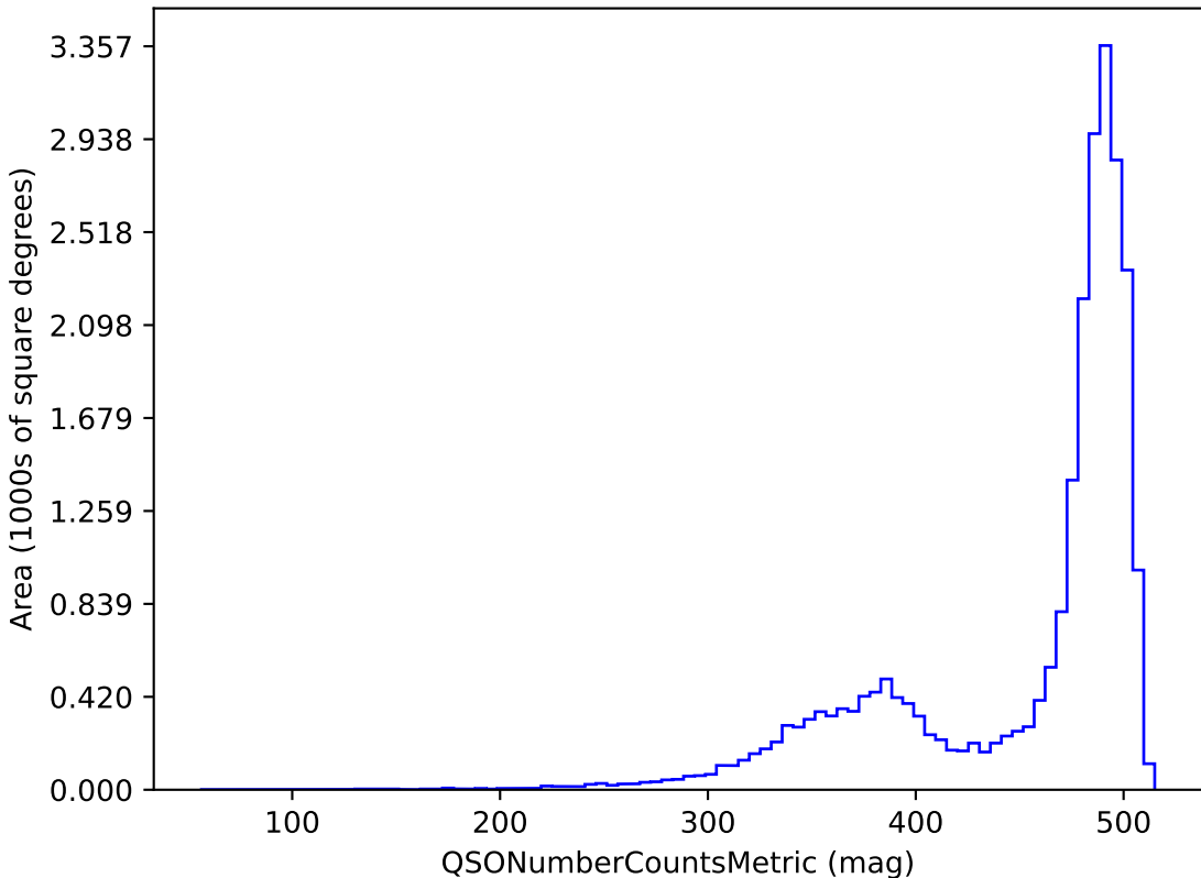
roman_v3.3_10yrs z band and non-DD: QSONumberCountsMetric
