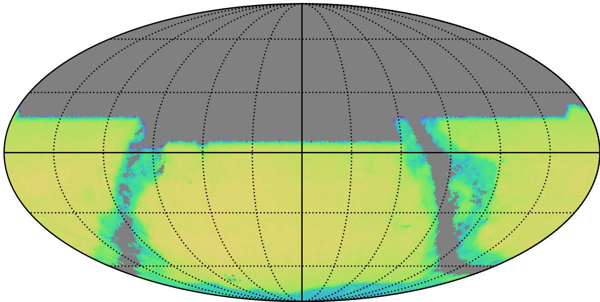
roman_v3.3_10yrs y band and non-DD: QSONumberCountsMetric
