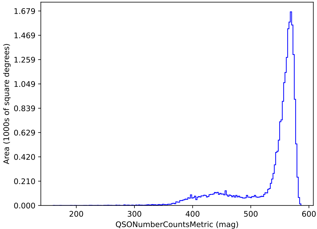
roman_v3.3_10yrs y band and non-DD: QSONumberCountsMetric
