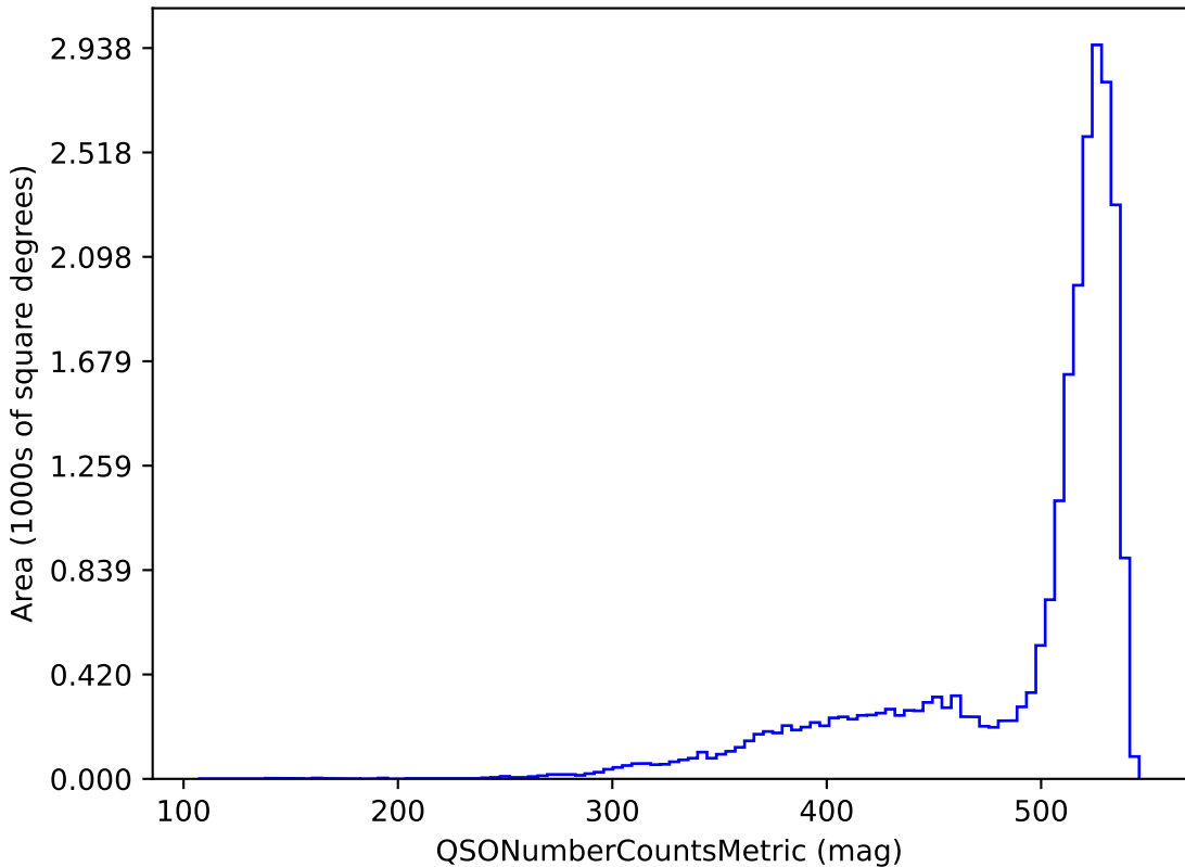
roman_v3.3_10yrs r band and non-DD: QSONumberCountsMetric
