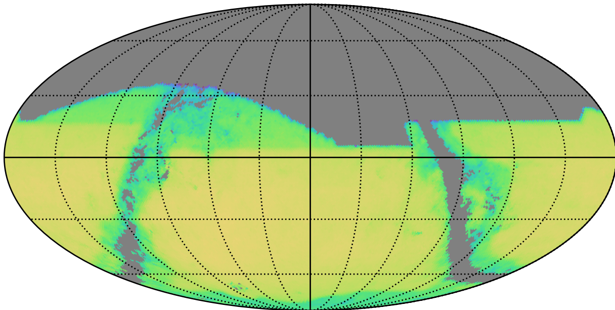
roman_v3.3_10yrs i band and non-DD: QSONumberCountsMetric
