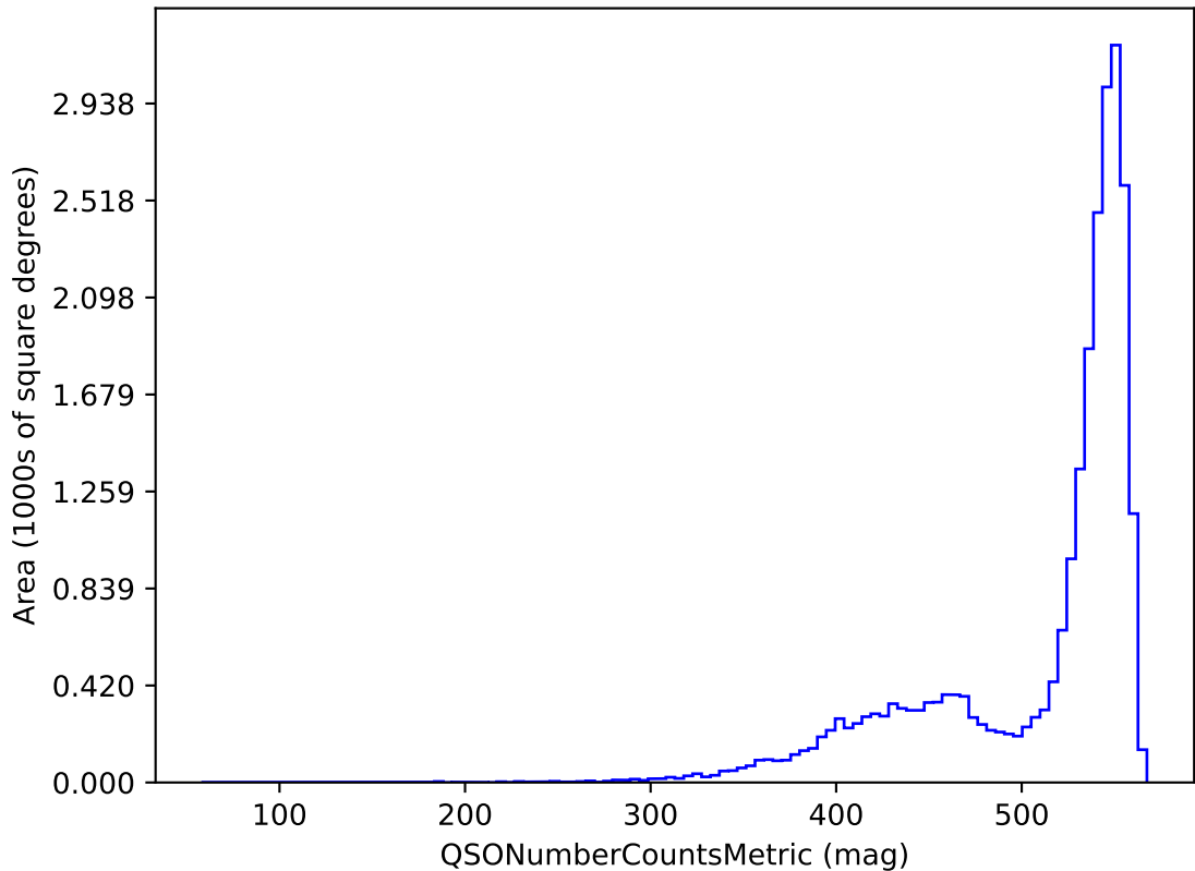
roman_v3.3_10yrs i band and non-DD: QSONumberCountsMetric
